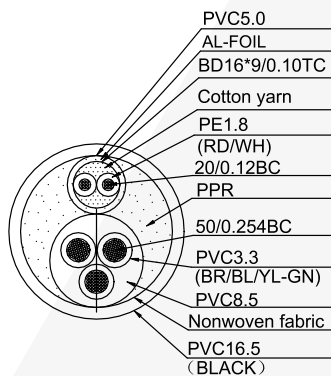
CABLE SECTION (8/1)
